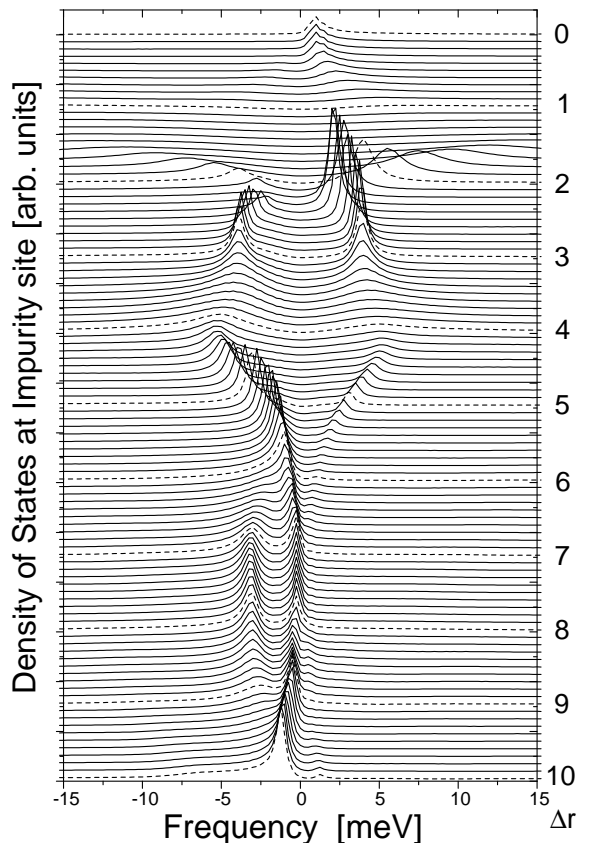
FIG. 1: DOS at \mathbf{R} = (0,0) as a function of \Delta r for two identical impurities with U_0 = 700 meV located at \mathbf{r}_1 = (0,0) and \mathbf{r}_2 = (\Delta r, 0) . The lattice constant is set to a_0 = 1 .
